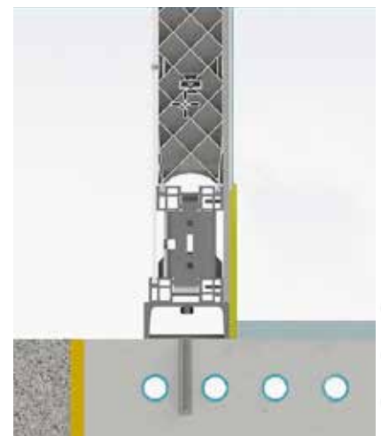
Anchoring system with ice dam
