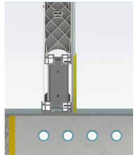
Installation into ice with steel plates
